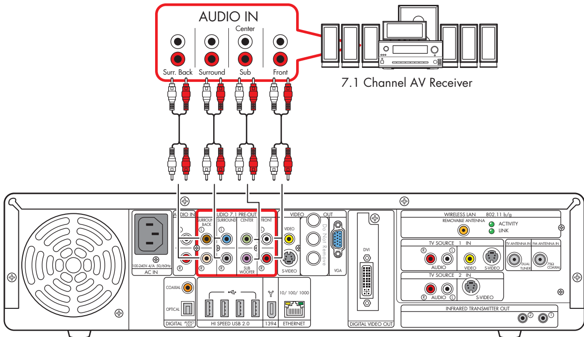
7.1 multichannel audio system connection
